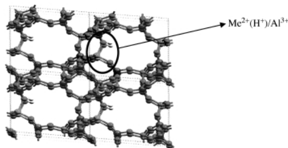
Figure 1. Structure of a 2+ dopant ion, charge-compensated by an acid proton, that replaces a framework \text{Al}^{3+} ion in AIPO-34, described using periodic boundary conditions.
